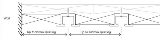
Double Recessed Curtain Tracks
